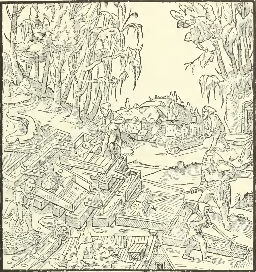
A—LAUNDER. B—CROSS TROUGH. C—TWO SPOUTS. D—BOXES. E—PLATE. F—GRATING. G—SHOVELS. H—SECOND CROSS TROUGH. I—STRAKE. K—WOODEN SCRUBBER. L—THIRD CROSS TROUGH. M—LAUNDER. N—THREE-TOOTHED RAKE.
